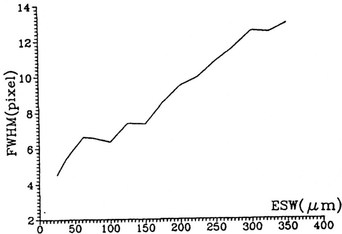
Fig. 2. The dependence of FWHM of the instrumental profile on ESW
