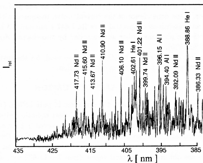
Fig. 2. Spectrum of the discharge in wavelength region 385 - 435 nm with laser interaction with \text{Nd}_2\text{O}_3 pill.
