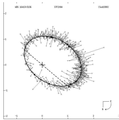
Figure 4: Outer orbit for the system HD 150680.
