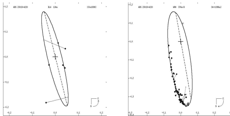
Figure 5: Inner and outer orbits for the system HD 217675/6.
