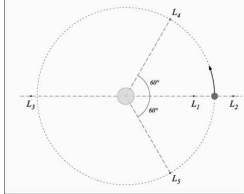
Figure 4: The restricted three body problem in a rotating coordinate systems with the two primaries on fixed position at the x-axis. The two stable equilibrium points L_4 and L_5 form triangles with the primaries.
